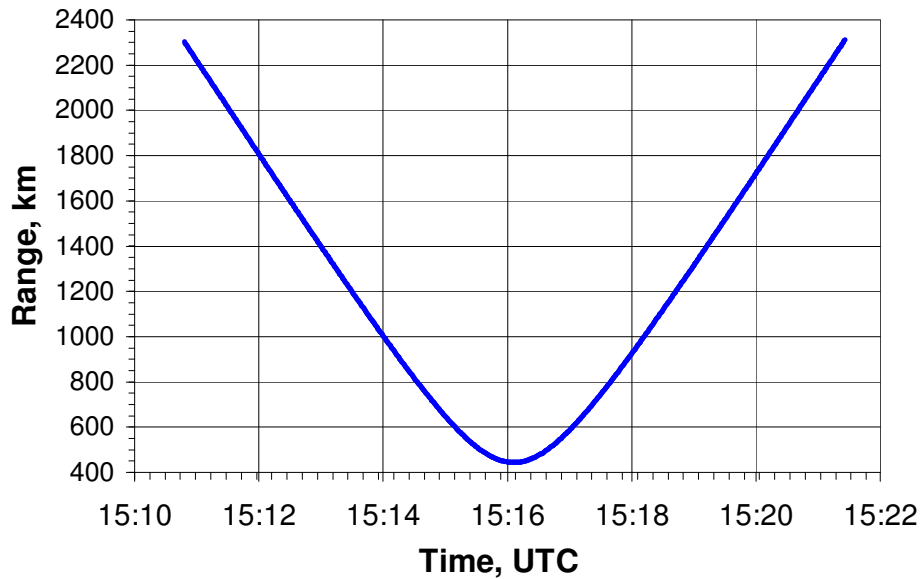
Range vs. Time
